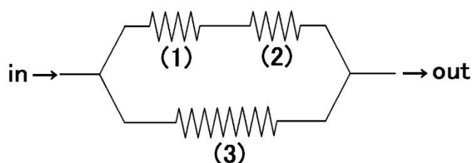
Parallel shunt (ZY-1) Connection diagram
